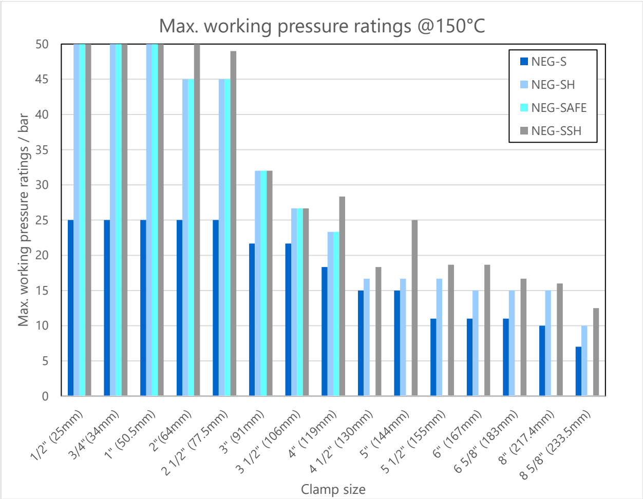
Figure 2: Maximum working pressure ratings for clamp sizes from 1/2" up to 8 5/8"
