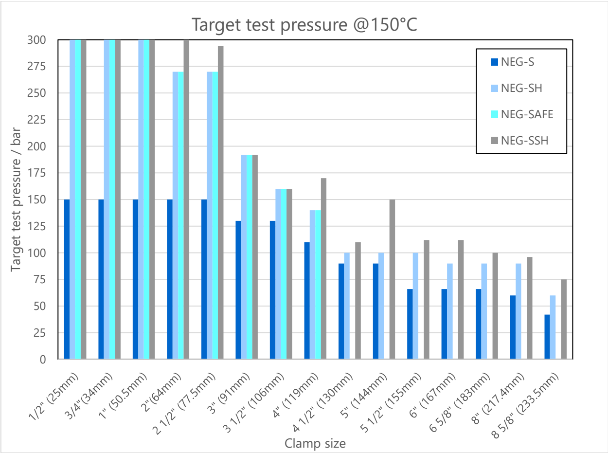
Figure 1: Target test pressure for clamp sizes from 1/2" up to 8 5/8"
