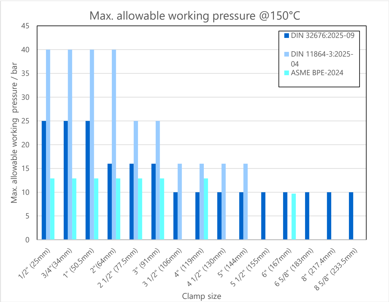
Figure 3: Maximum allowable working pressure according to various common standards for clamp sizes from 1/2" up to 8 5/8"
