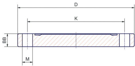
Blind Male Flange
