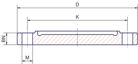
Blind Male Flange
