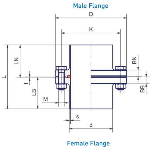
Blind-Female Flange
